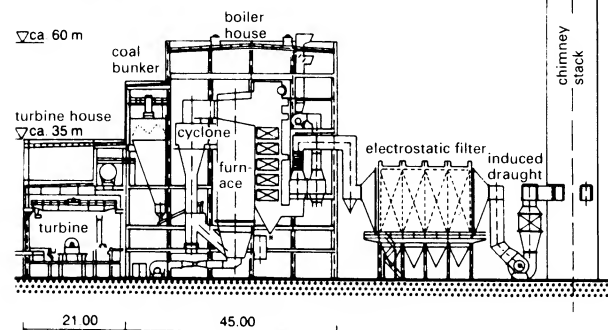
3 Cross-section of the power station shown in the plan view
